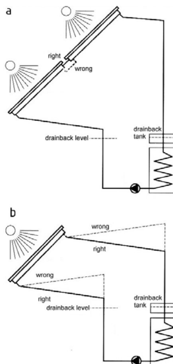
Fig. 1: Examples of correctly, respectively wrongly designed drainback collector loops showing the basic principle of this technology and some of its constraints.
