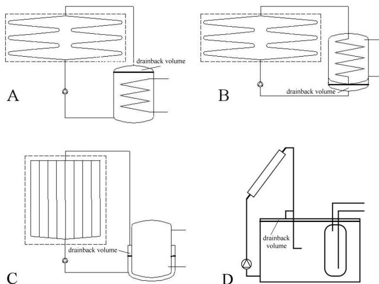
Fig. 2: Different implementations of the drainback concept.
