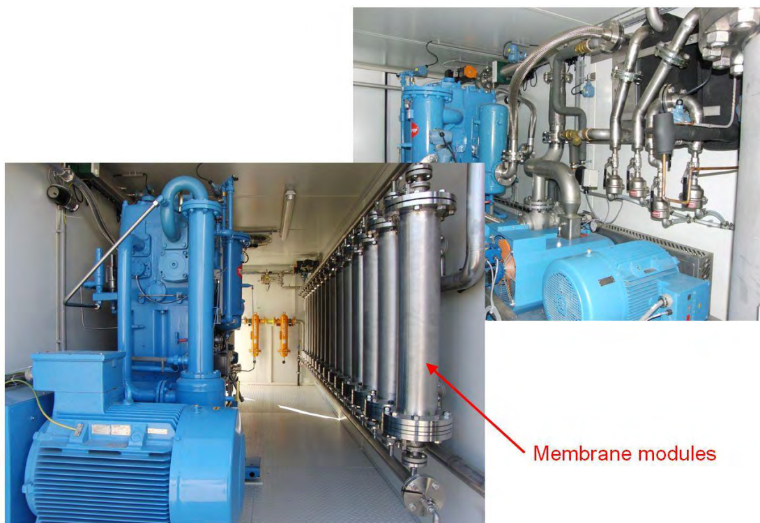
Figure 5: Recent start-up of first AXIOM plant in Germany
